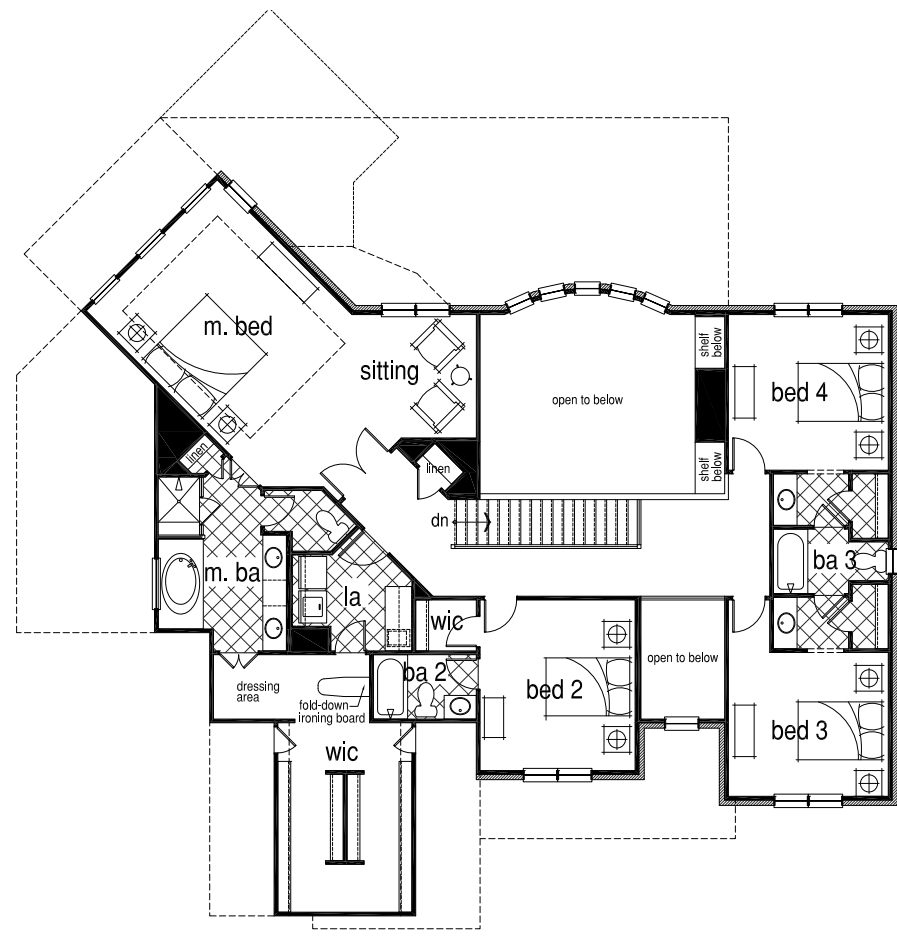
Upper Level
