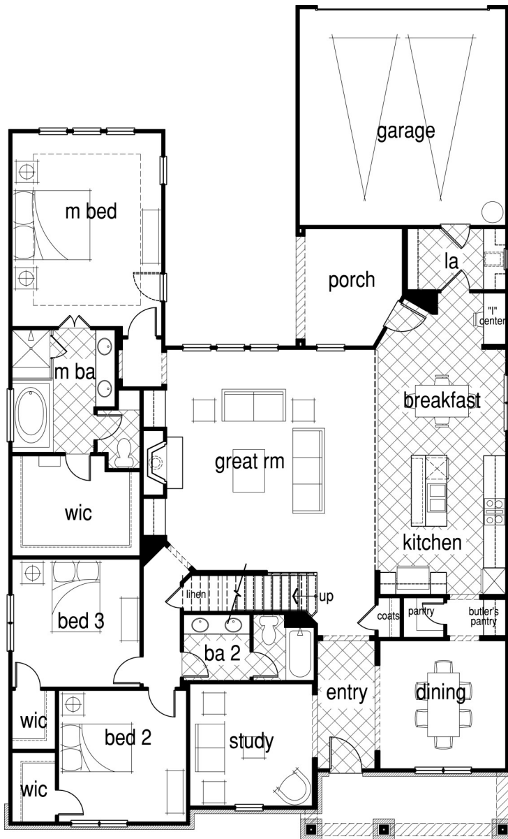
floor plan
