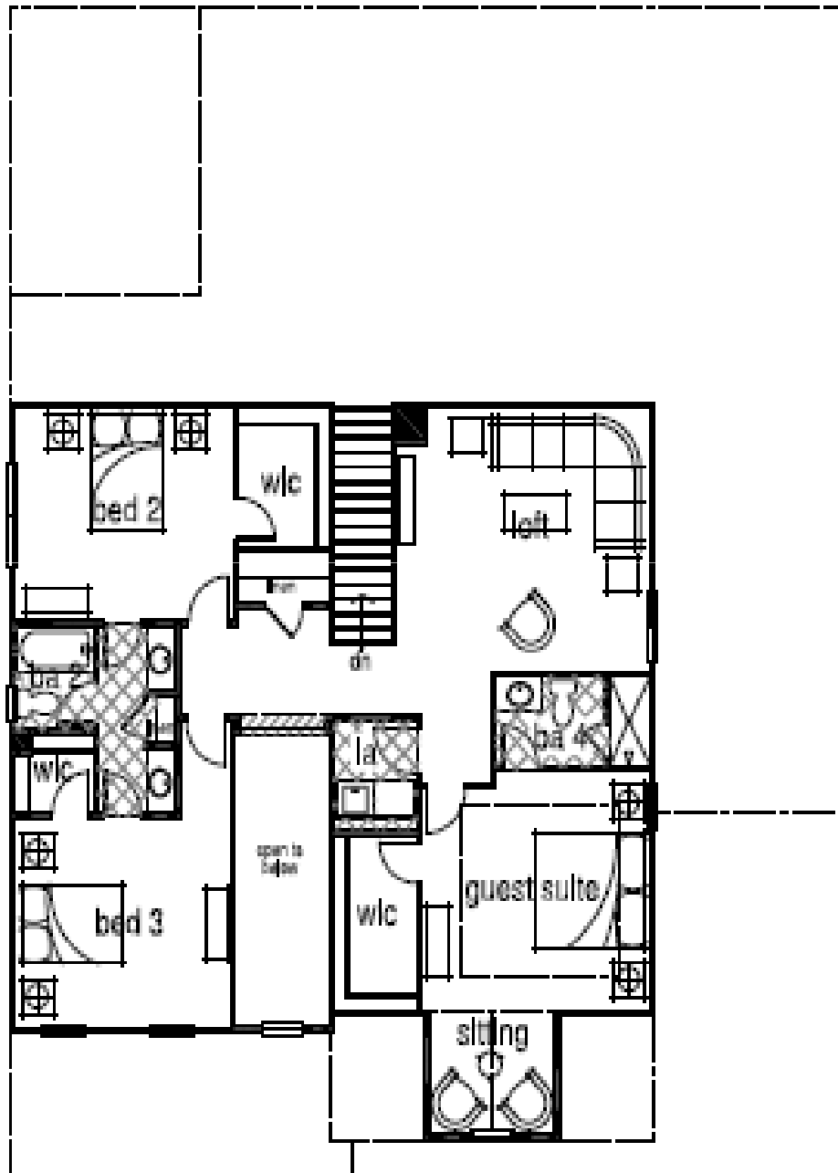
Second Floor Aspen
